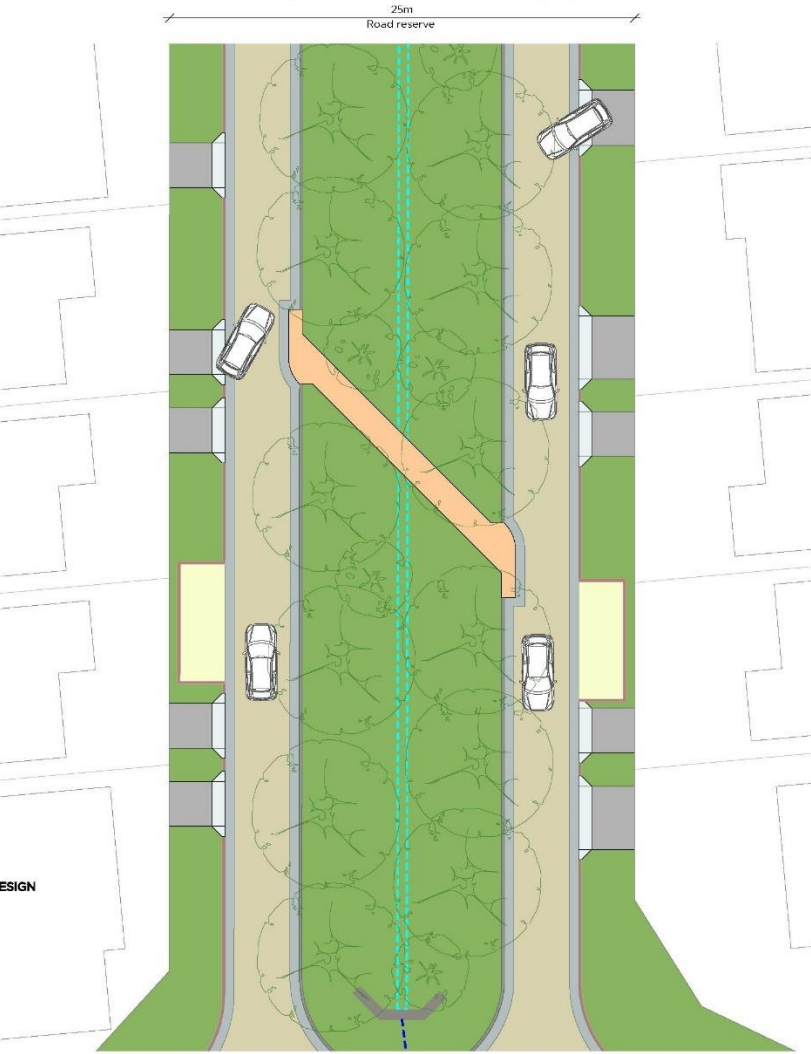
Figure 66: Swale Street I - section and plan
