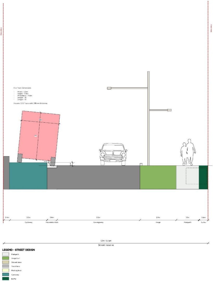
Figure 49: Edge Street - details
